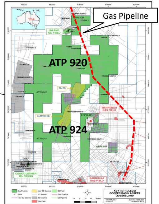
Location of ATP 920 and ATP 924 in the Cooper Eromanga Basin and zoomed in area showing location of Carpentaria Gas Pipeline
