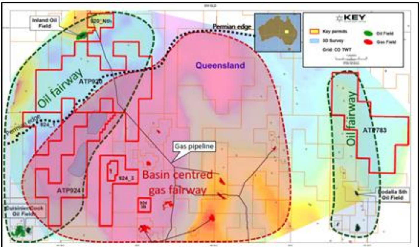
Location of Permian gas fairway (red) and oil fairway (green) in relation to ATP 920 and ATP 924
